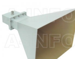
LB-650-15-C-7/16F Standard Gain Horn Antenna 1.12-1.7GHz 15dB Gain 7/16(DIN) Female
